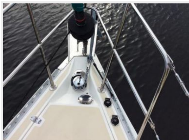
Bow Windlass Lumar
