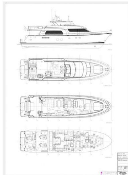
General Arrangement
