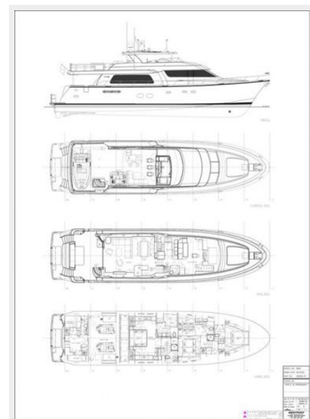
General Arrangement
