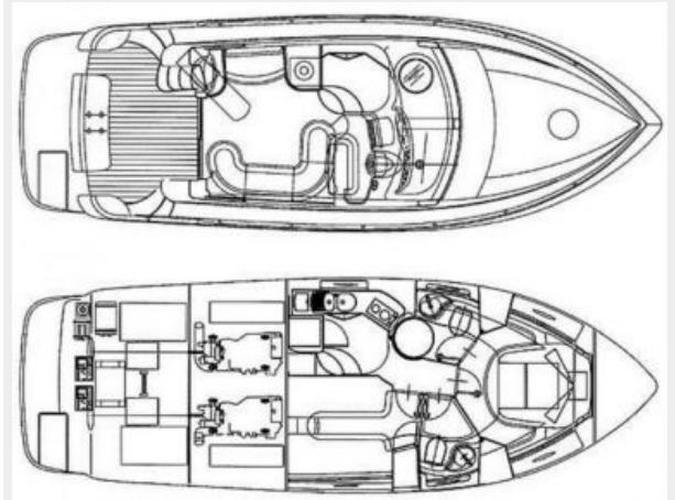
Manufacturer provided image-floor plan
