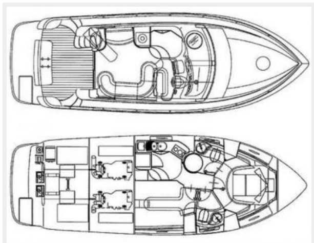
Manufacturer provided image-floor plan
