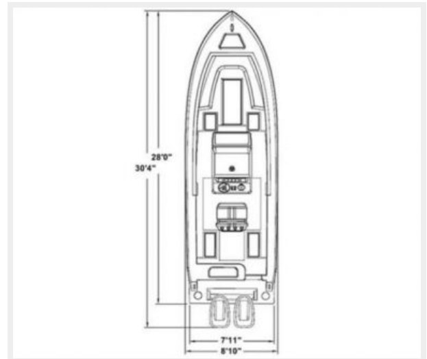
Layout view
