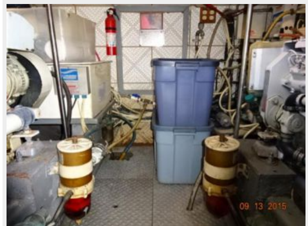
43' Marine Trader engine room forward
