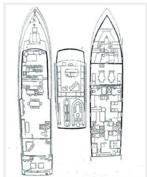
Layout Drawing
