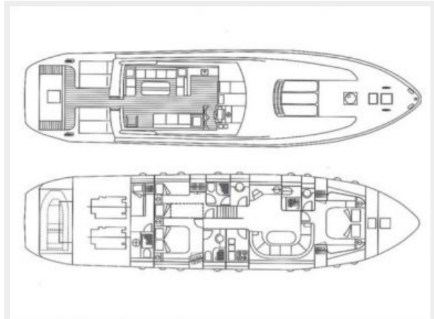
GA Plan
