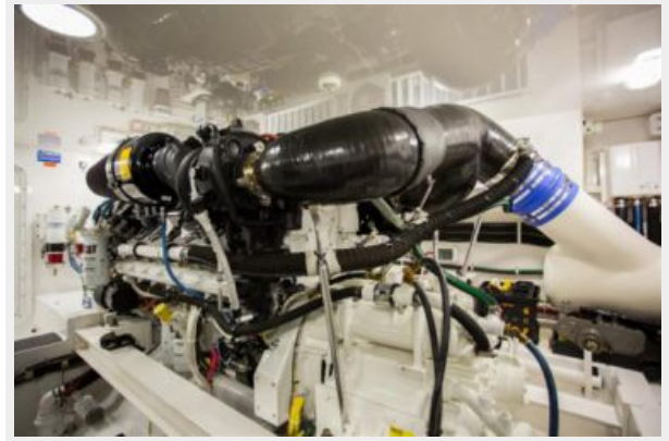
Starboard Engine
