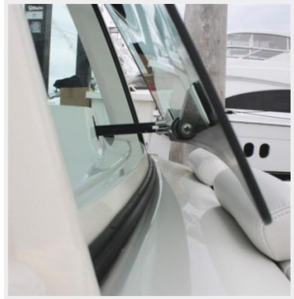
Windshield in Open position
