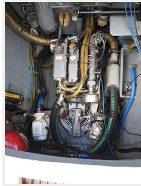
port engine room
