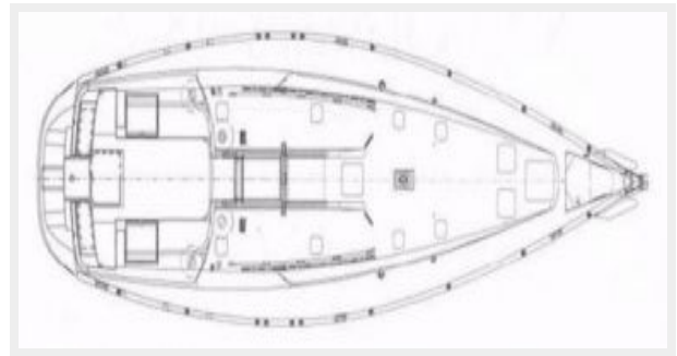
Deck Layout
