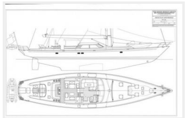
Cockpit Line Drawing
