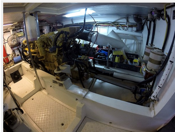
Prima 45 engine room starboard
