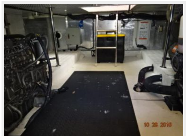
40' Albin engine room forward
