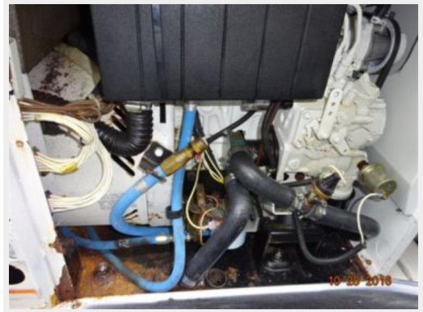
40' Albin generator
