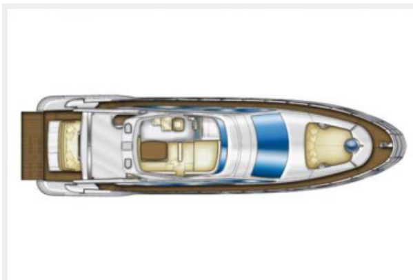
Flybridge Layout
