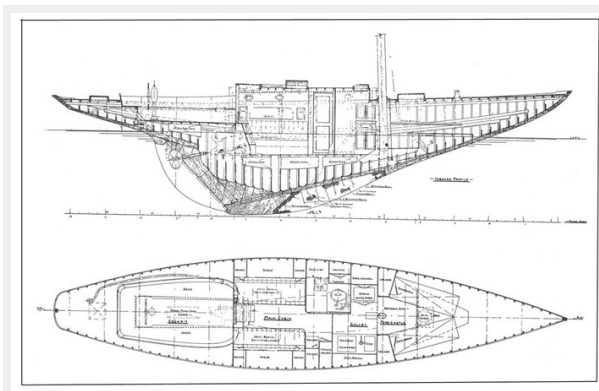
General Arrangement Plan
