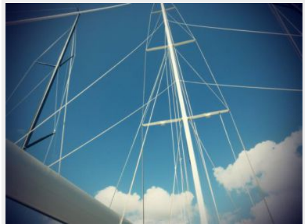
C & C 41 Keel Stepped Mast w/ Running Back Stays
