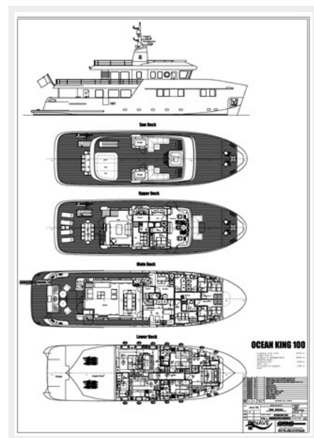
General Arrangement
