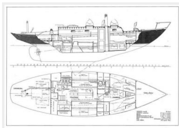
Arrangement Plan
