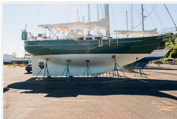
Full Keel w/ cutaway forefoot
