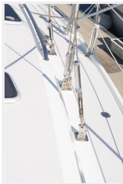
307 Port Stays
