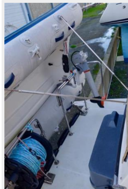
Tender Davit system
