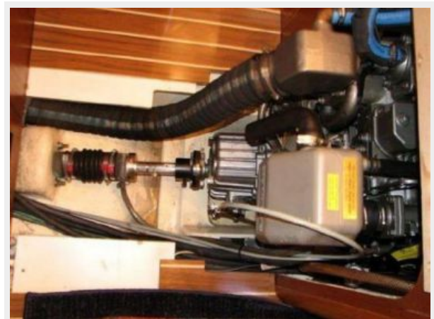
Dripless packing gland
