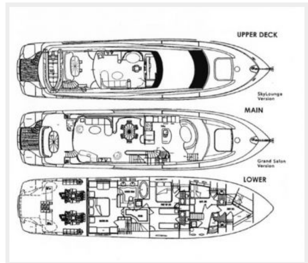
Layout Arrangements
