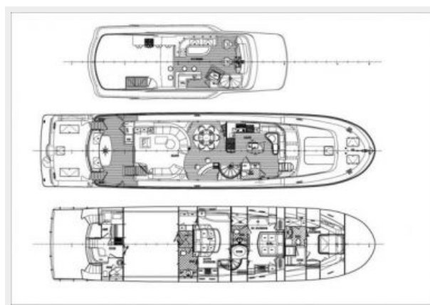
5017 GA Dwg
