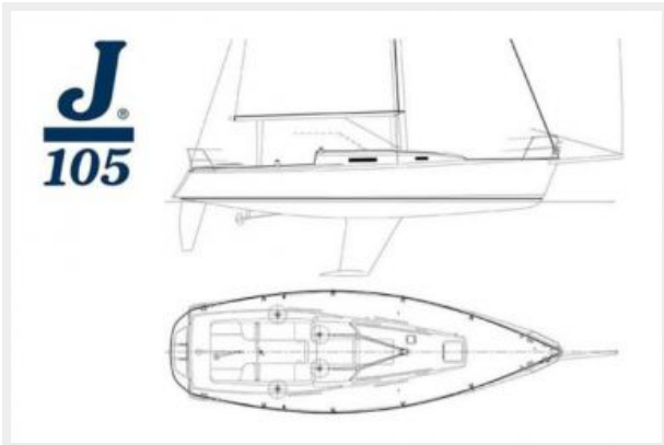
Deck Layout
