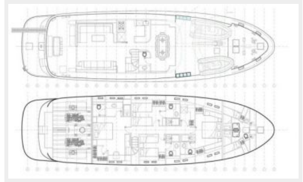
layout_main_lower_deck
