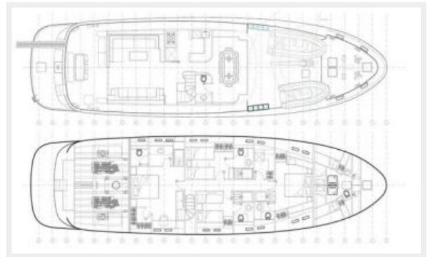
layout_main_lower_deck
