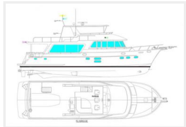
General Arrangement
