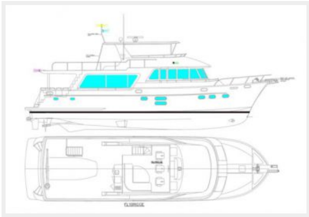
General Arrangement
