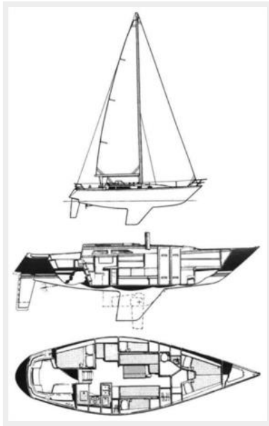
c&c_40-2_drawing
