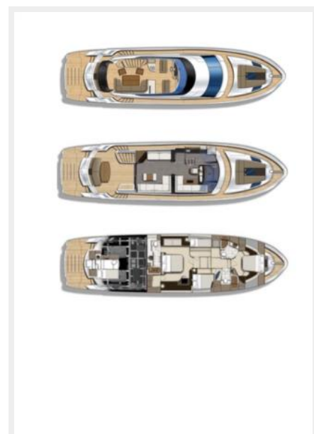
Marquis 630 Deck plans
