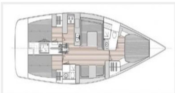
Interior Plan
