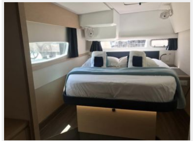
EventuallyInt2LR
