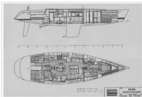
56-041 General Arrangement
