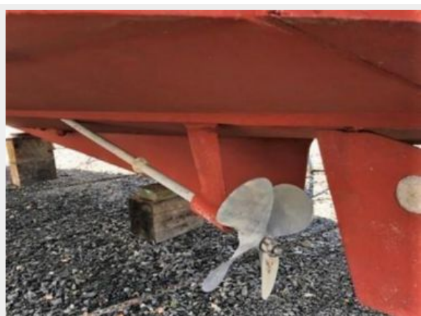
Port Side Propeller & Rudder
