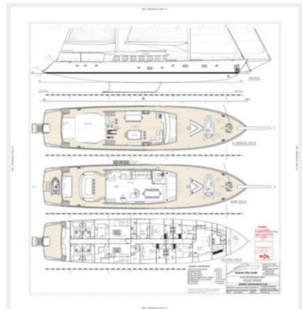
General arrangement Plan-50
