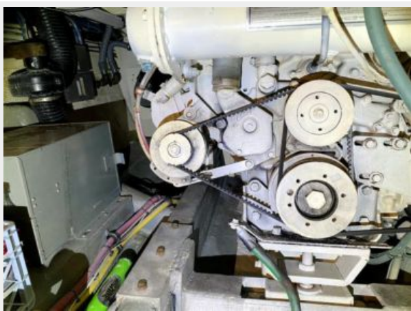
starboard CAT 3208TA Diesel engine
