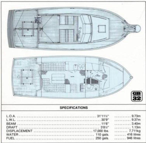
Grand Banks 32 Sedan Layout
