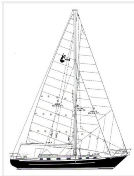
Crealock44ProfileSailplan
