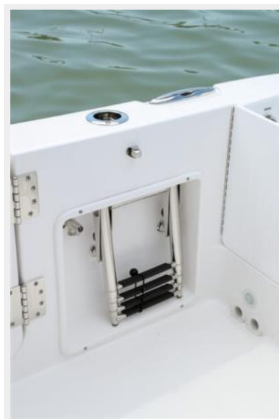
EdgeWater-262cx-Dive-Door-Ladder-Storage-with-Raw-Water-Washdown
