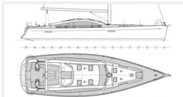
pilot-saloon55-layout-deck
