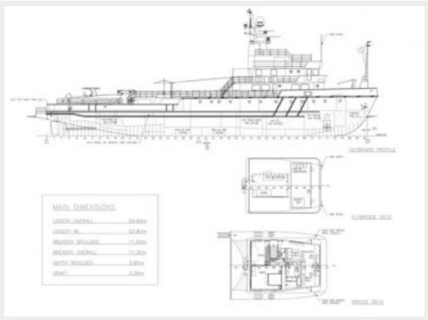
General Arrangement Post 2019 Refit 1
