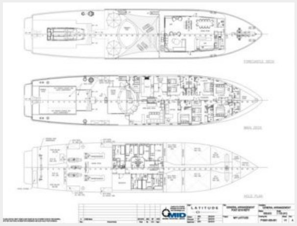
General Arrangement Post 2019 Refit 2
