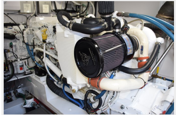
Newer engine mounts, Airseps
