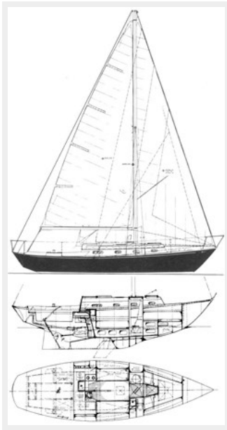
corvette_31_drawing
