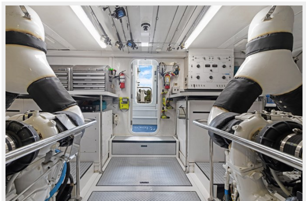
BELLA GIORNATA 94' Lazzara 2000/2018 Flybridge Motor Yacht: Engine Room
