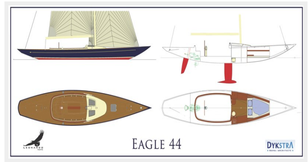
eagle44_layout
