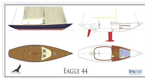
eagle44_layout
