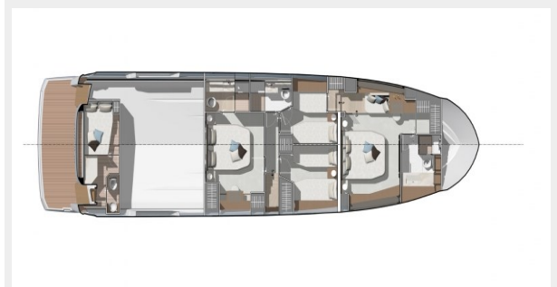
X70 Layout 4 CabinsBD_d
