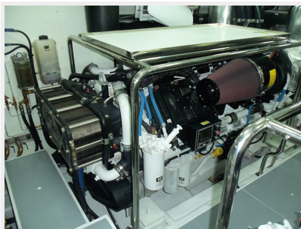
Starboard engine
